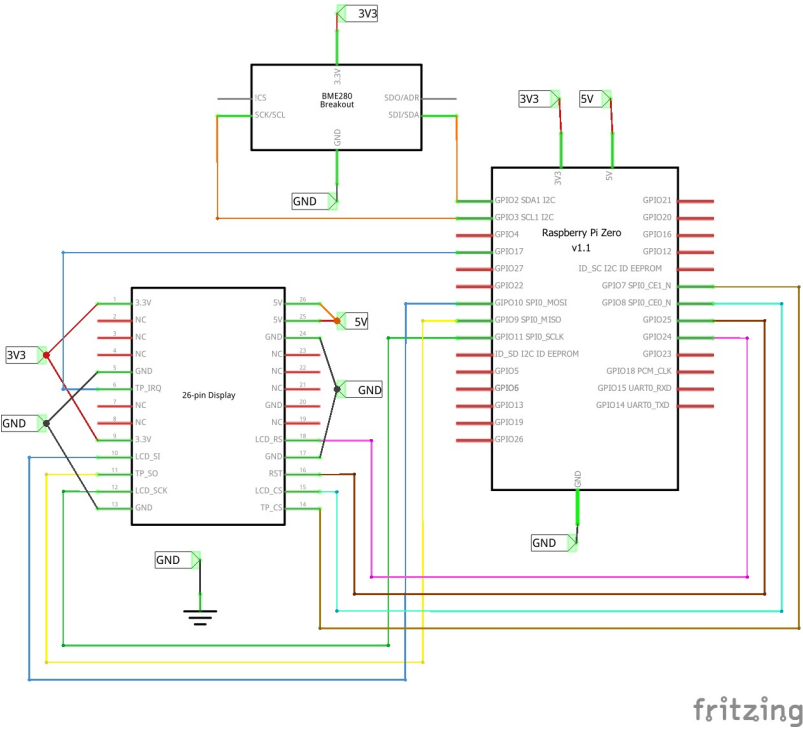
Figure 45: Control Station System Schematics
