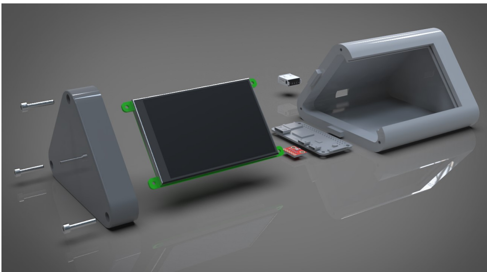
Figure 53: Control Station Exploded Axonometric
