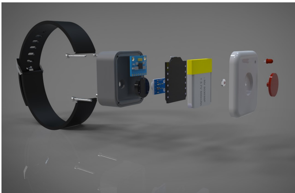
Figure 51: Bracelet Exploded Axonometric
