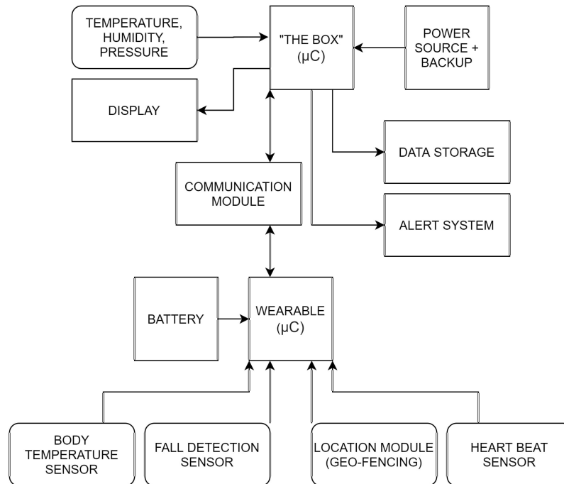
Figure 42: Components Schematics
